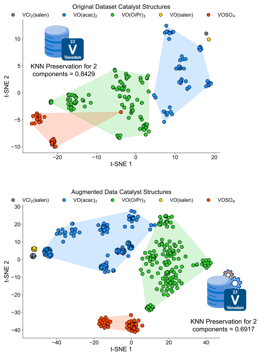
Figure A1. ESA data distribution t-SNE plots before and after DA using 2 components.
